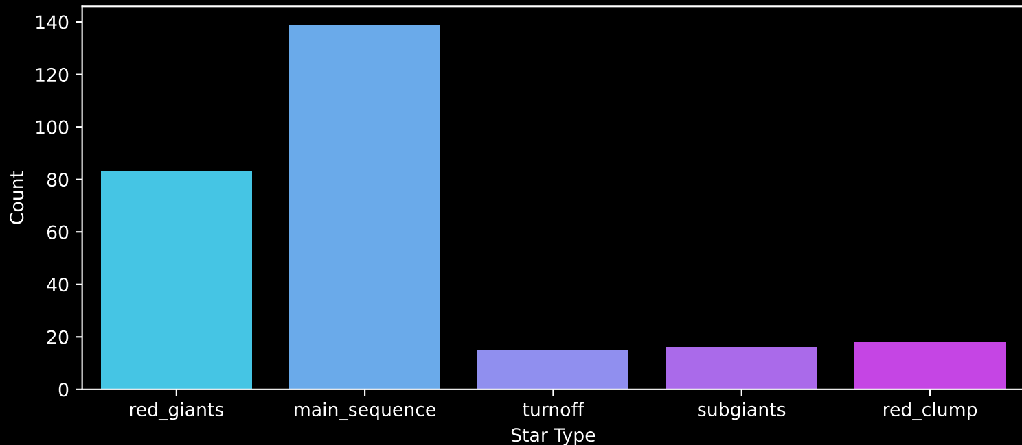
APOGEE DR17 Field: [178+36_btx] Count plot of Star Type
