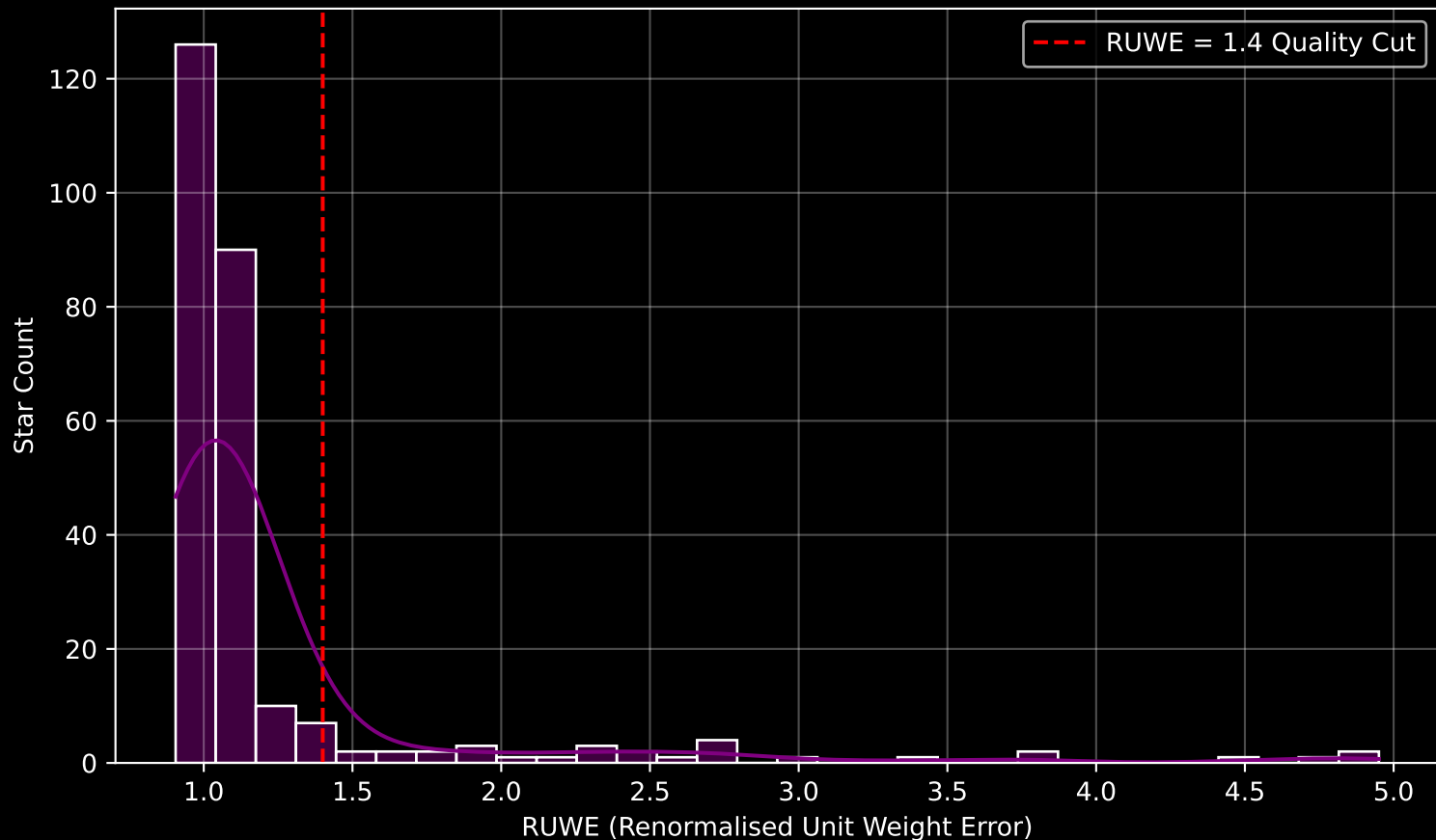
GAPOGEE DR17 Field [178+36_btx] RUWE Distribution (n= 262)
