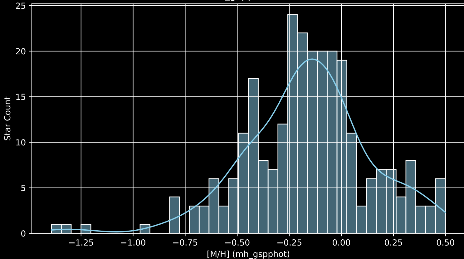
APOGEE DR17 Field: [178+36_btx [M/H] (mh_gspphot) (n= 267)
