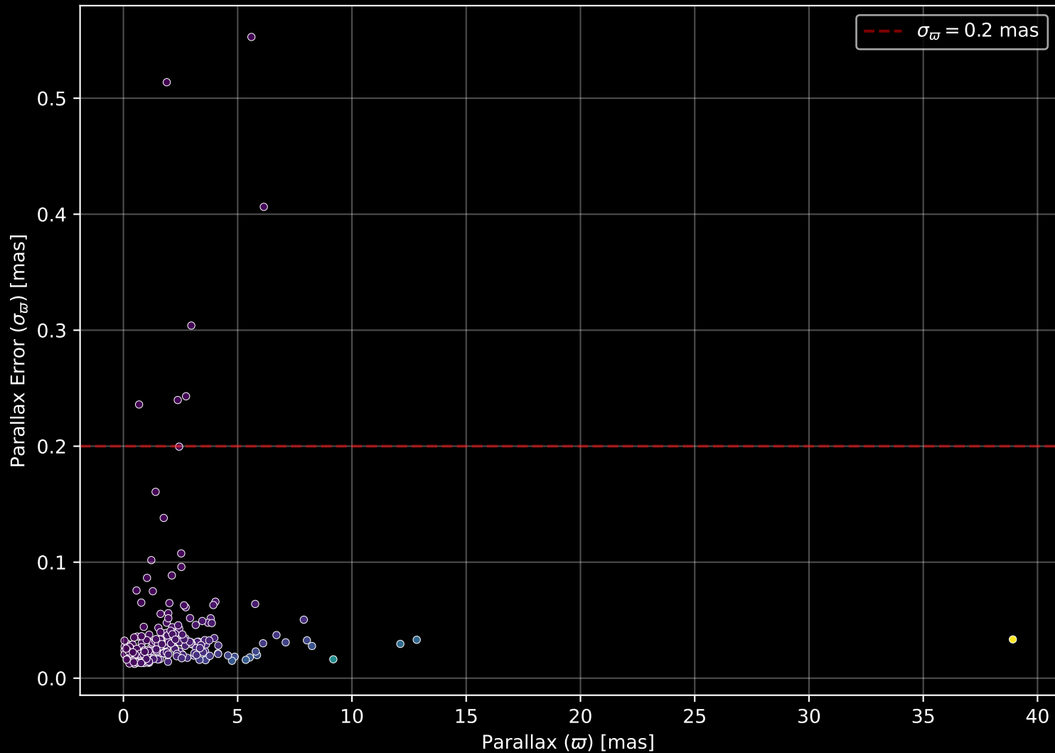
APOGEE DR17 Field: [178+36_btx] Parallax Quality (n= 271)
