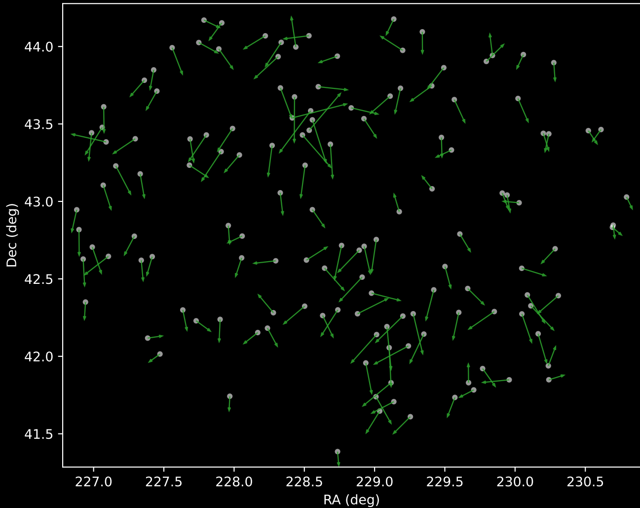
APOGEE DR17 Cluster 4 Proper Motion Vectors (n=138)
