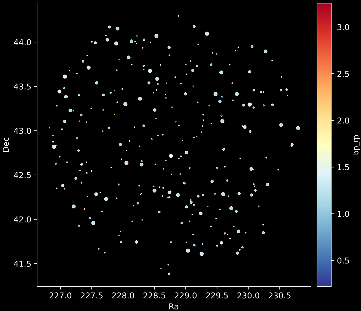
APOGEE DR17 Field: [178+36_btx] Stars: 271
