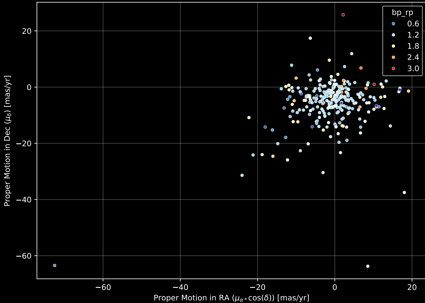
APOGEE DR17 Field: [178+36_btx] Proper Motion Diagram (n= 271)
